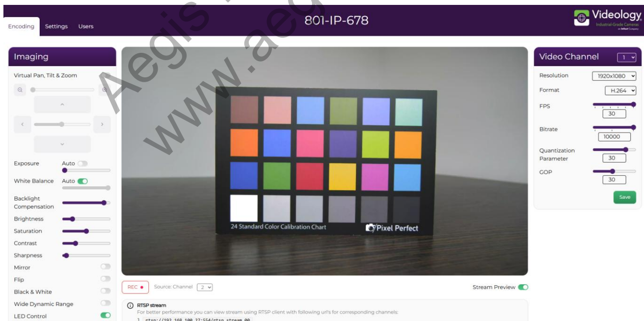
Figure 2 Web Interface
