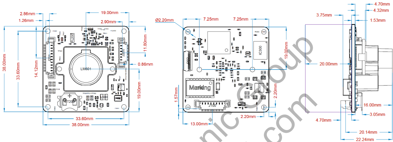
Figure 28 Camera Dimensions
