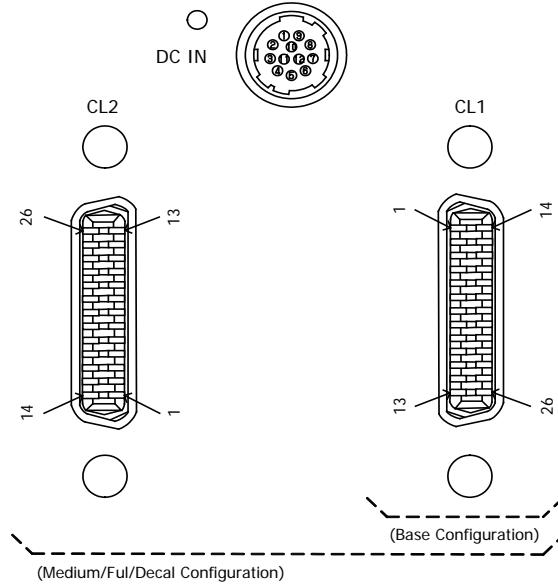
Connector (CL1)
