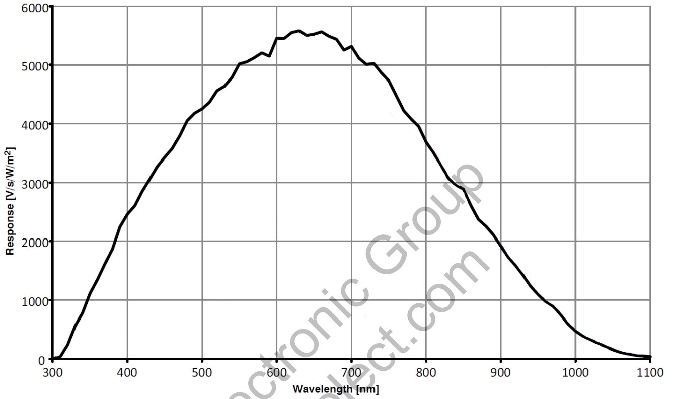
Spectral Response Curve
