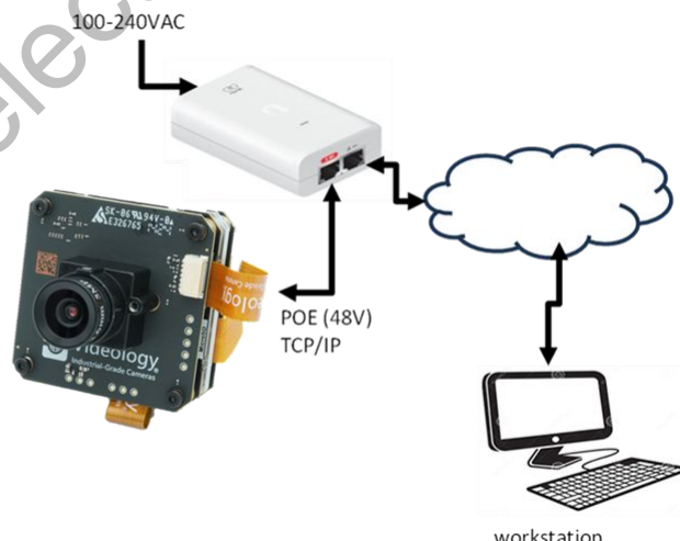
Basic setup SCAiLX-CAM with PoE
