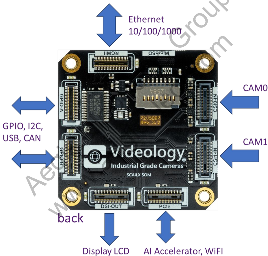
SCAiLX-SOM-AI board connectivity
