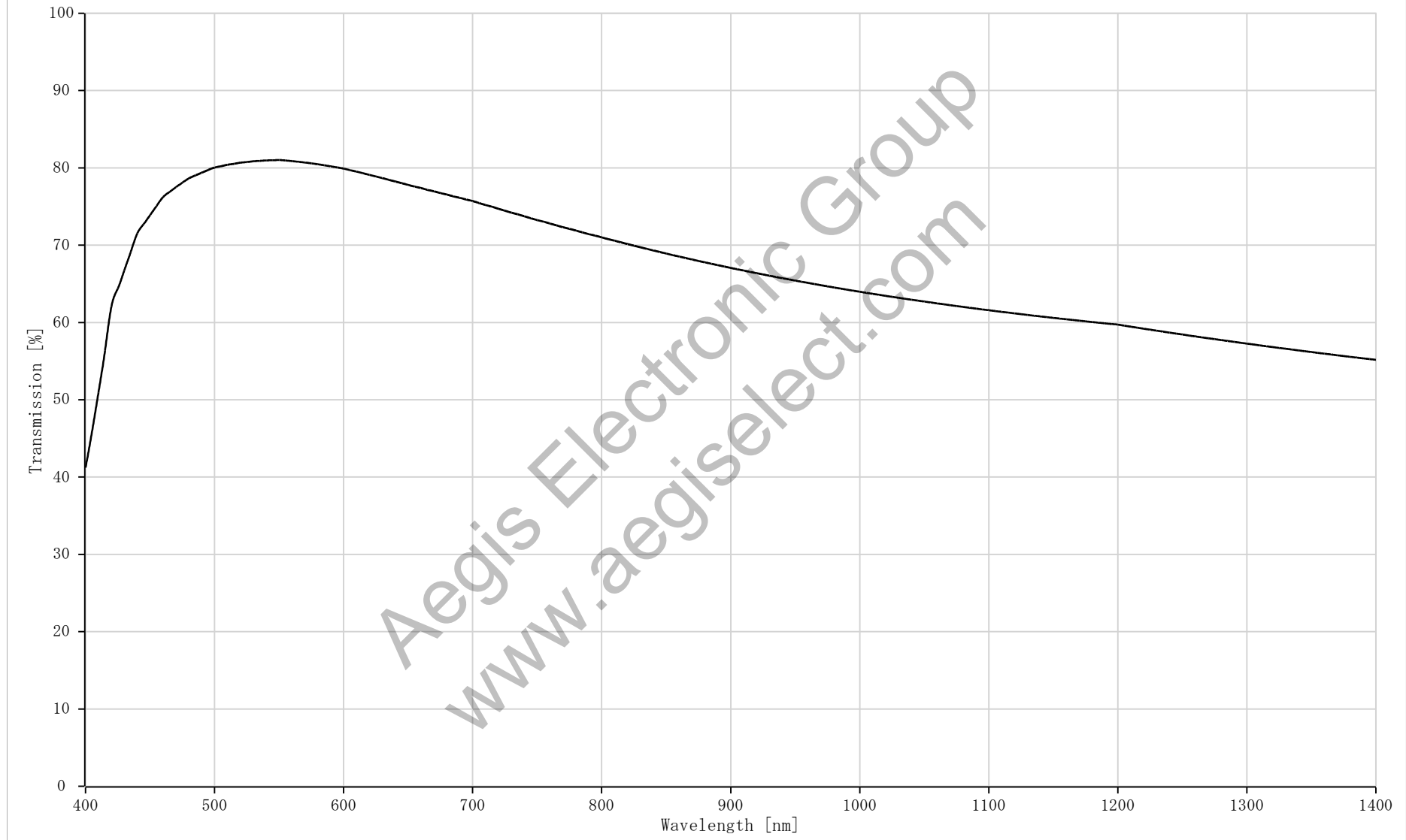
LM15FC-R Transmission
