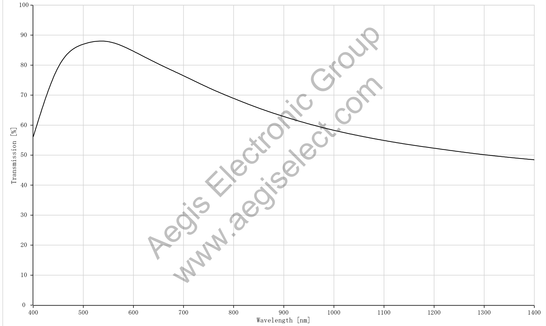
LM16EC-IR Transmission
