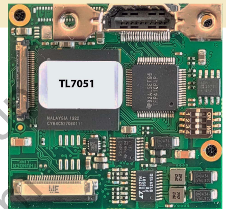
Image for reference only. TL7051 does not have a HDMI connector assembled.
