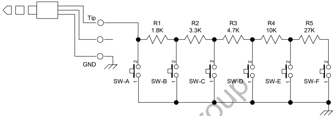
SW board circuits for 3.5Φ stereo jack (External SW)
