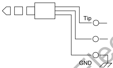
3.5Φ stereo jack pin assignment for communication
